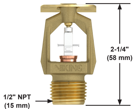
Figure 2: Sprinkler Dimensions
