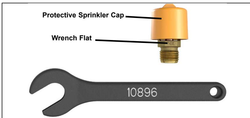
Figure 1: Standard Sprinkler Wrench 10896W/B
