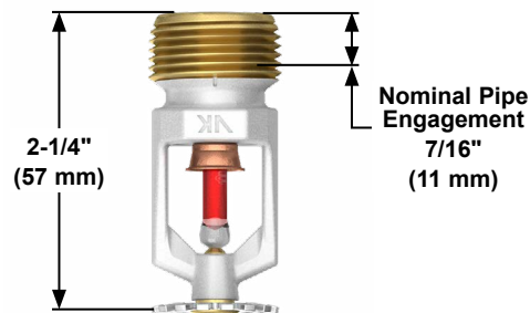
Figure 2: Sprinkler Dimensions
