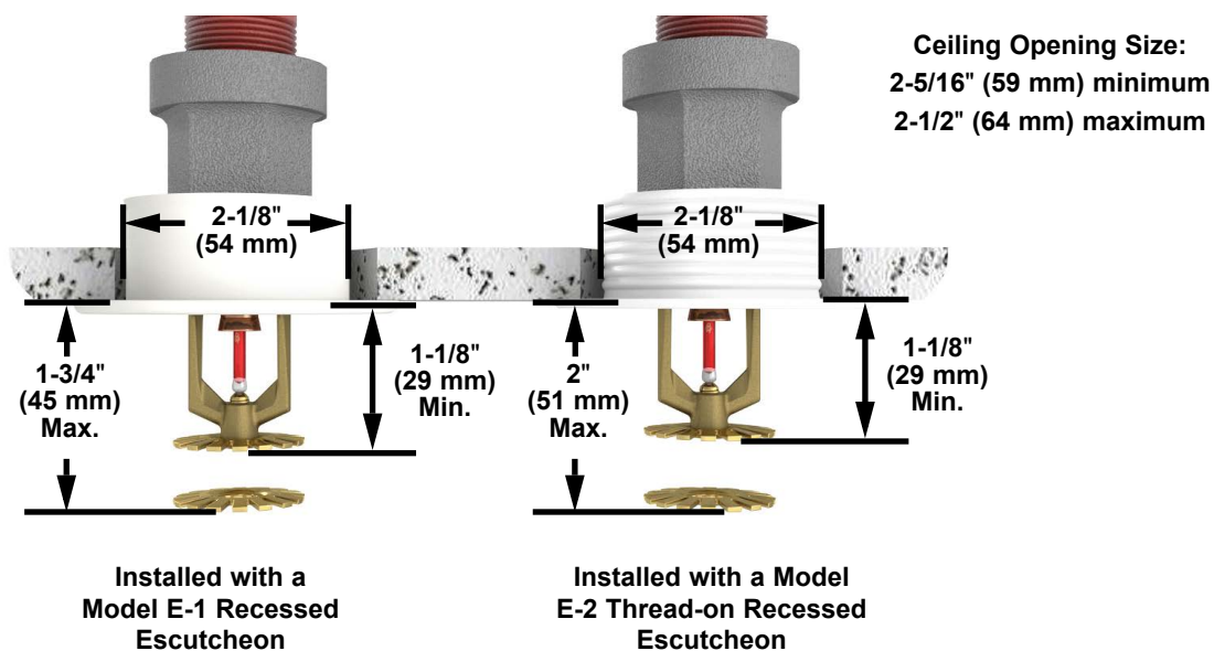
Figure 4: Sprinkler Dimensions with the Model E-1 and E-2 Recessed Escutcheons
