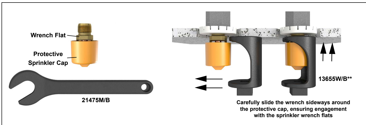
Figure 1: Sprinkler Wrenches
