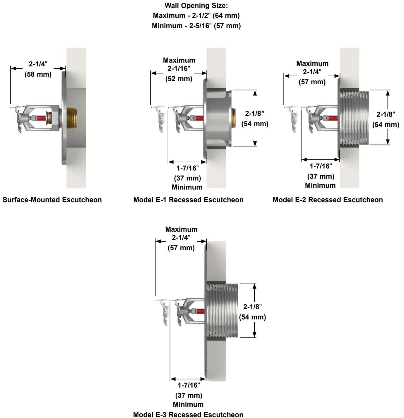
Figure 4: Installation Dimensions with Escutcheons
