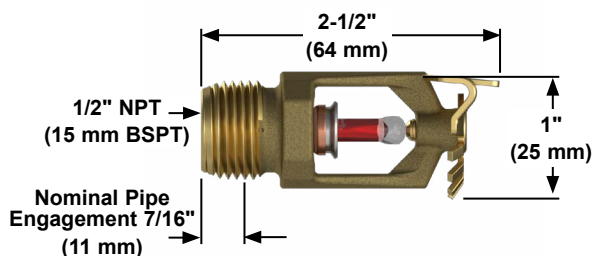
Figure 2: Sprinkler Dimensions
