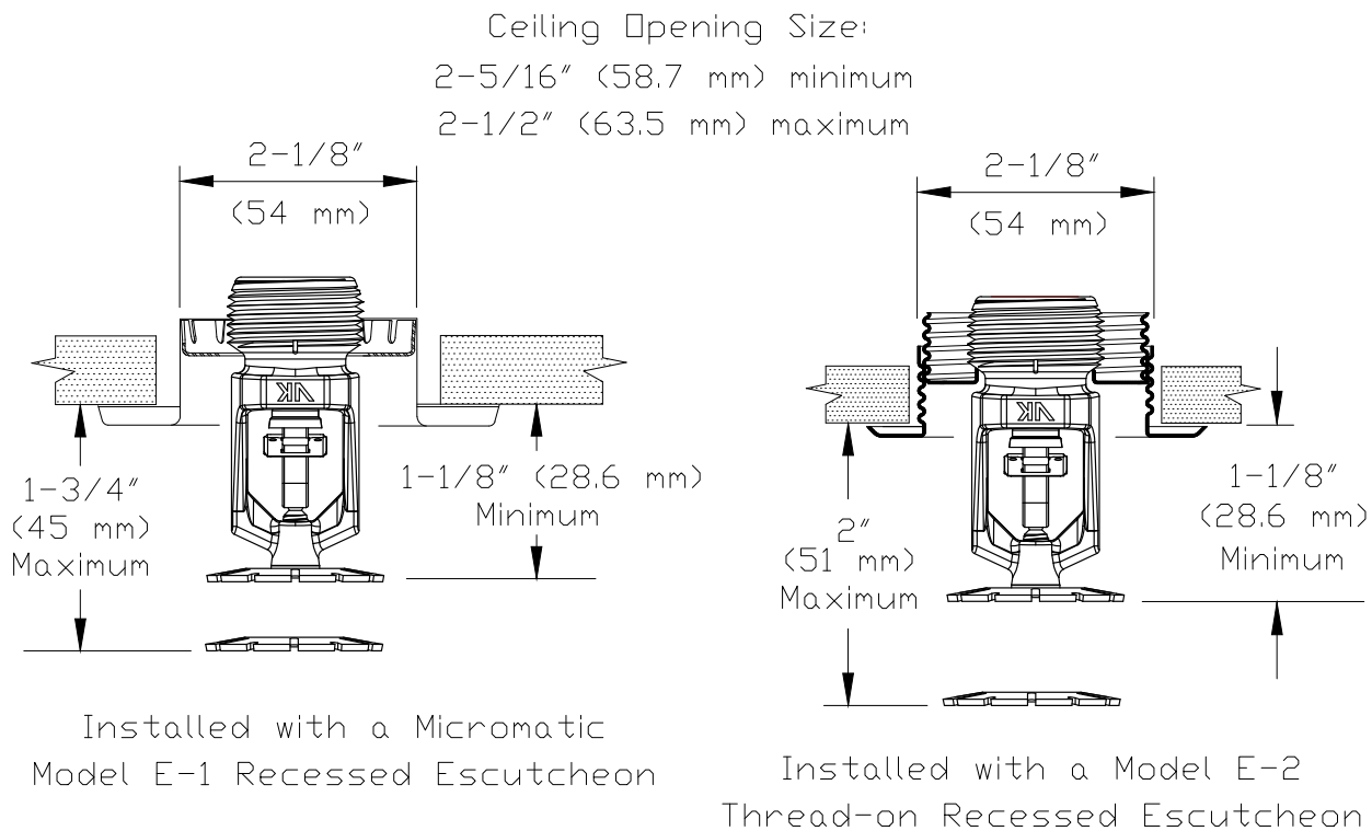
Figure 4: Sprinkler VK603 Dimensions with the Model E-1 and E-2 Recessed Escutcheons
