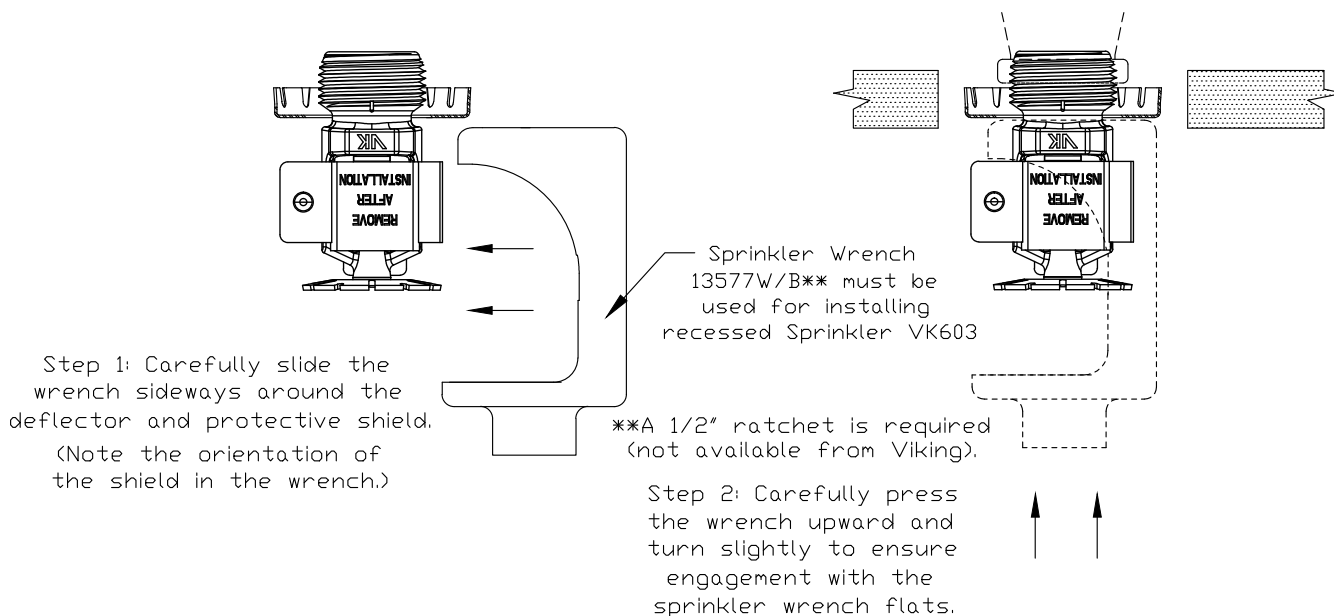
Figure 2: Wrench 12144W/B for Coated and/or Recessed Pendent Sprinklers
