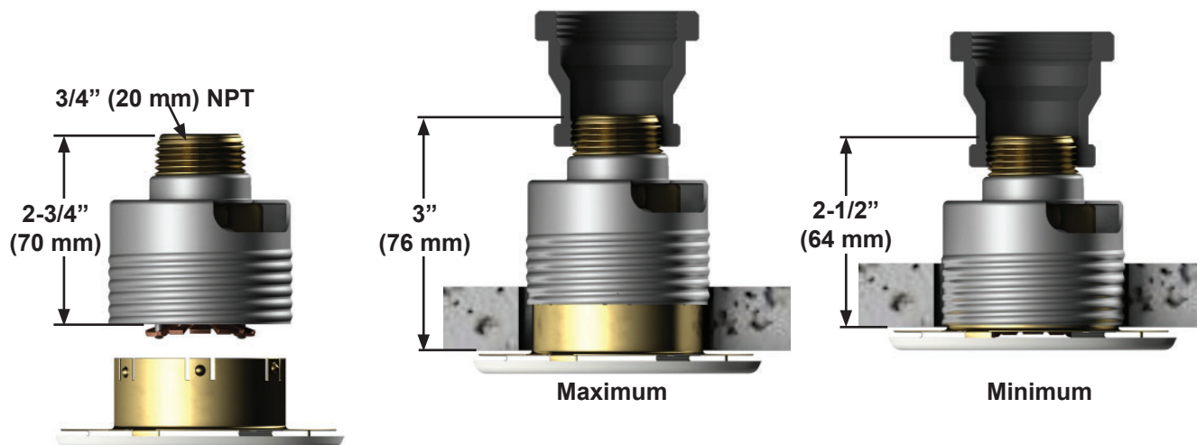
Figure 3: Sprinkler Installation Dimensions
