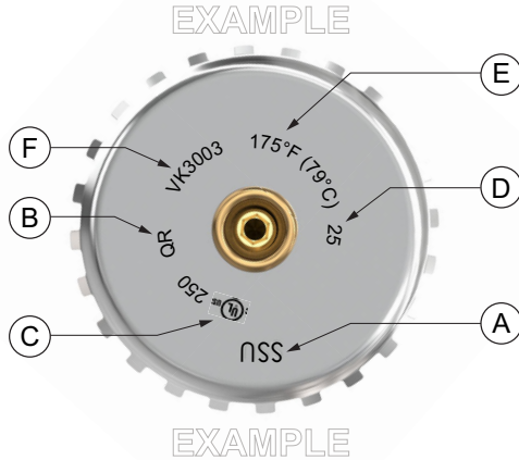
Figure – 1: Markings
