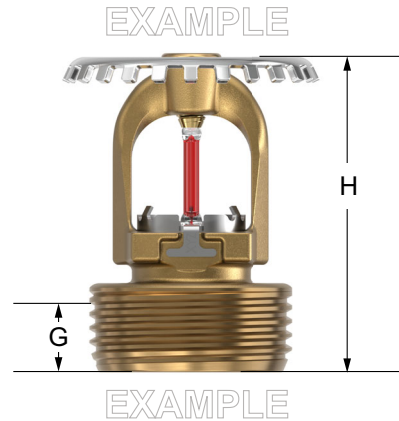
Figure – 2: Dimensions
