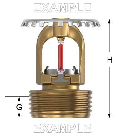
Figure – 2: Dimensions
