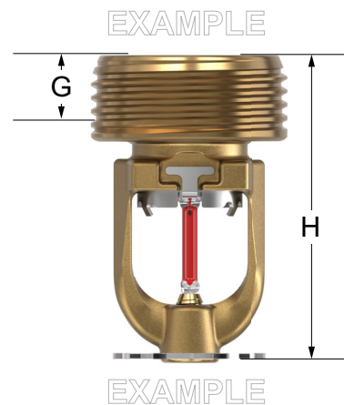
Figure – 2: Dimensions
