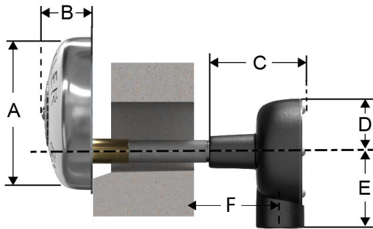
Figure – 1: Water Motor Alarm Dimensions
