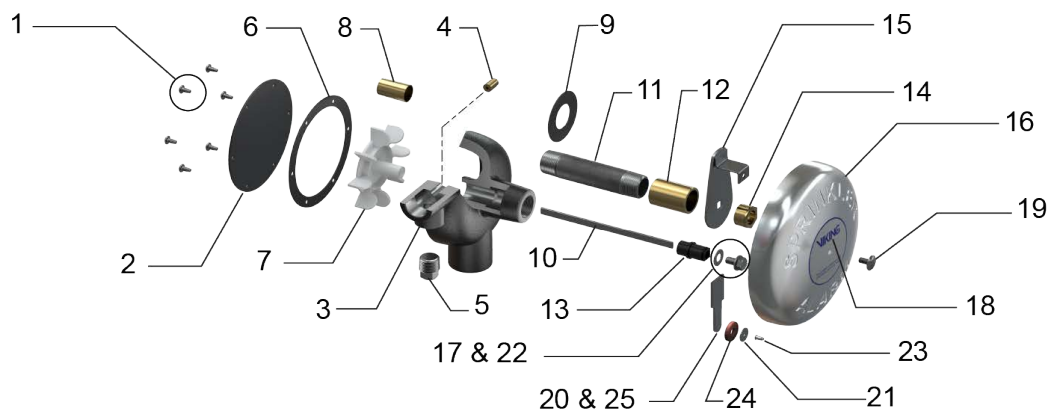
Figure – 4 Water Motor Alarm Components
