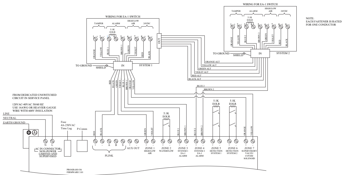
DETAIL A
