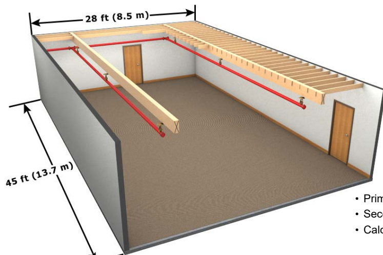
Figure 5: Alternate Entire Compartment Protection Scheme Example
