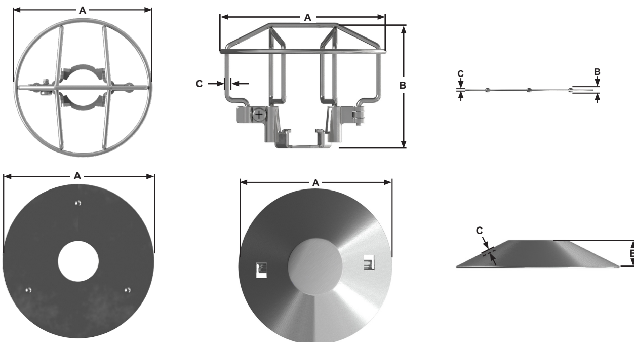
Figure 1: Dimensions
