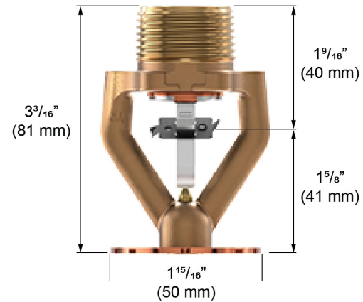
Figure – 2: Sprinkler Dimensions
