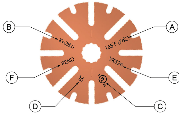
Figure – 1: Deflector Markings
