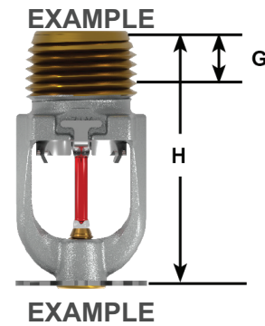
Figure – 2: Dimensions
