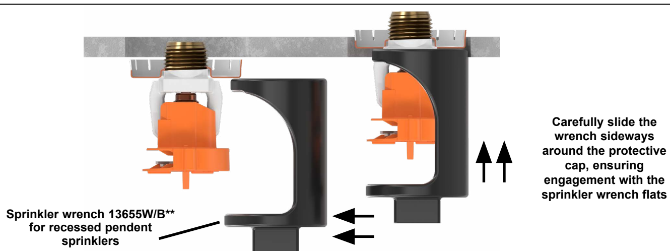
Figure 2: Installing Recessed Pendent Sprinklers ** A 1/2" ratchet is required (not available from Viking)
