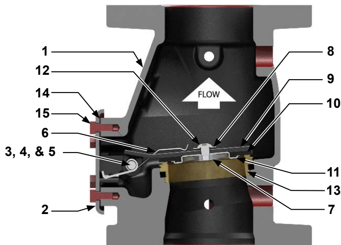
Figure 3 - Replacement Parts
