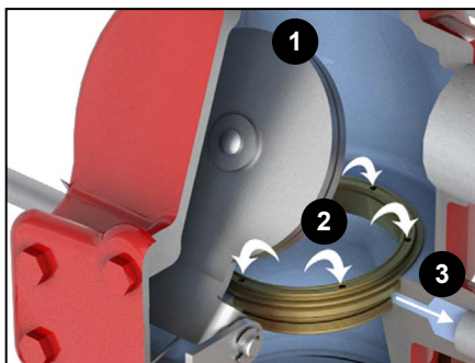
Figure 1 - Alarm Ports
