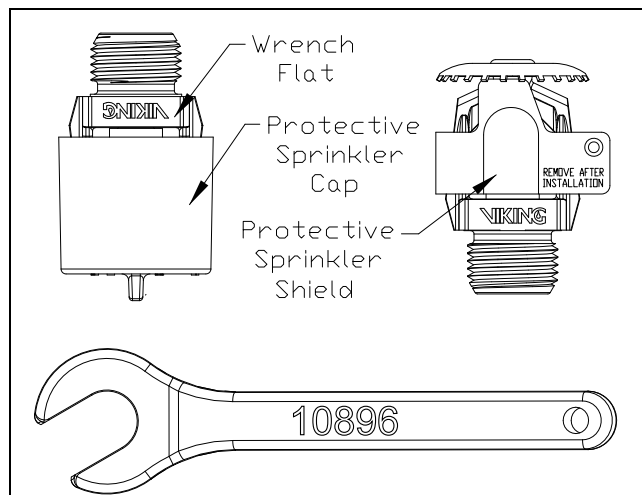
Figure 1: Standard Sprinkler Wrench 10896W/B
