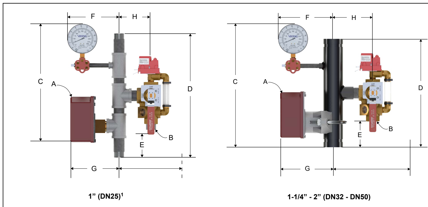
Figure 4 - Residential EasyPac with TESTanDRAIN and PRV
