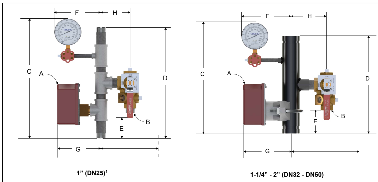
Figure 3 - Residential EasyPac with TESTanDRAIN
