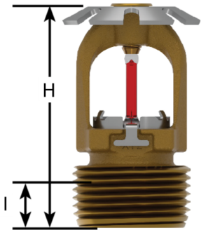
Figure – 2: Dimensions
