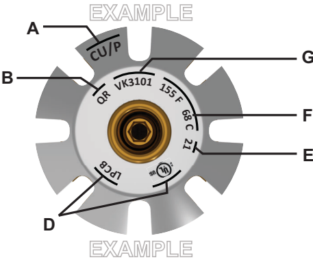
Figure – 1 Markings
