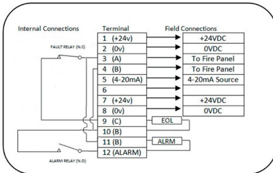
Figure 7: VSF303 UV/IR Internal Inter-connections
