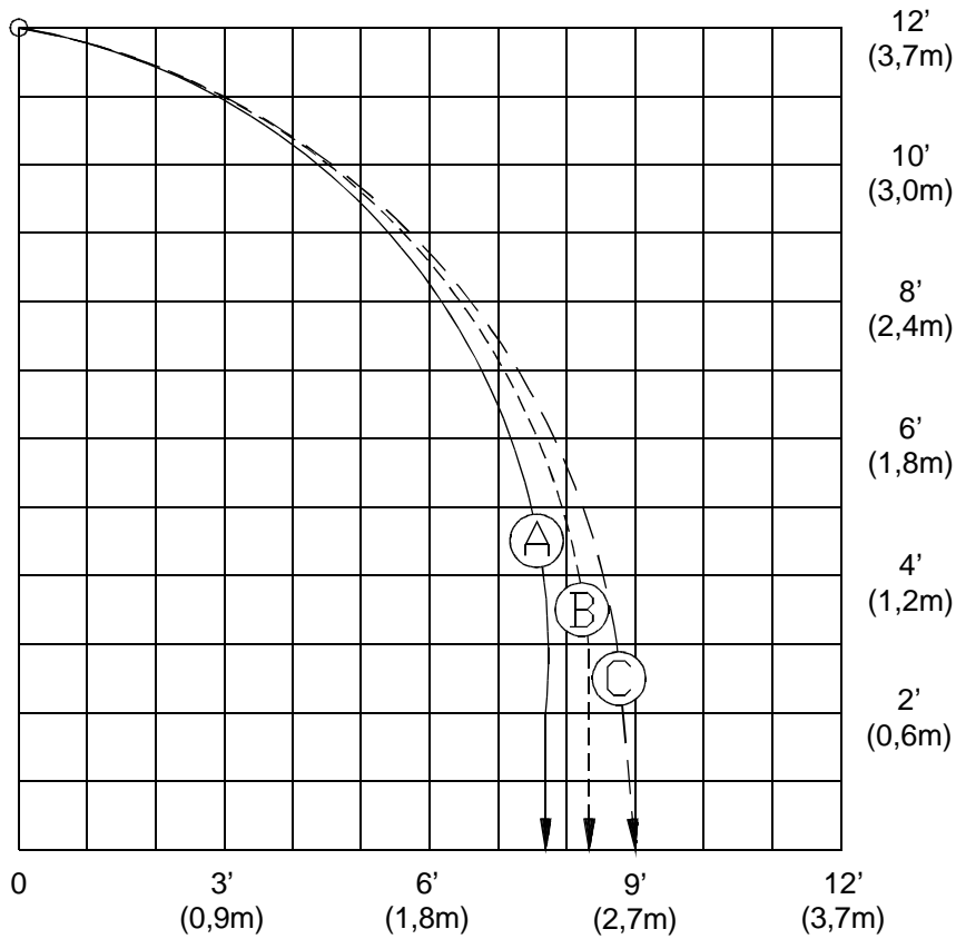
Typical profile of one half of the spray pattern produced by a Viking ESFR Pendent SIN VK500 Sprinkler (K=14.0)
