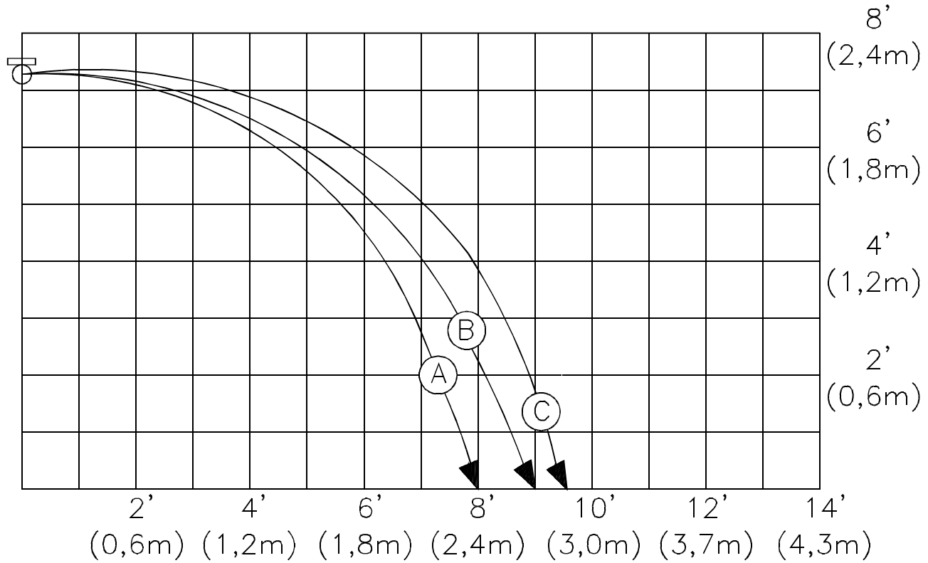
Typical profile of one half of the spray pattern produced by a Viking Micromatic® Model N-2 1/2" (15 mm) Upright Sprinkler SIN VK130 (Nominal K-Factor = 5.6 U.S.)
