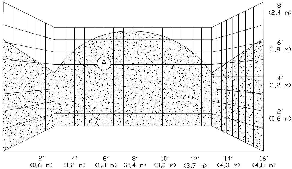
Typical profile of one half of the spray pattern produced by a Viking Model HQR-2 Institutional Extended Coverage Pendent Sprinkler
