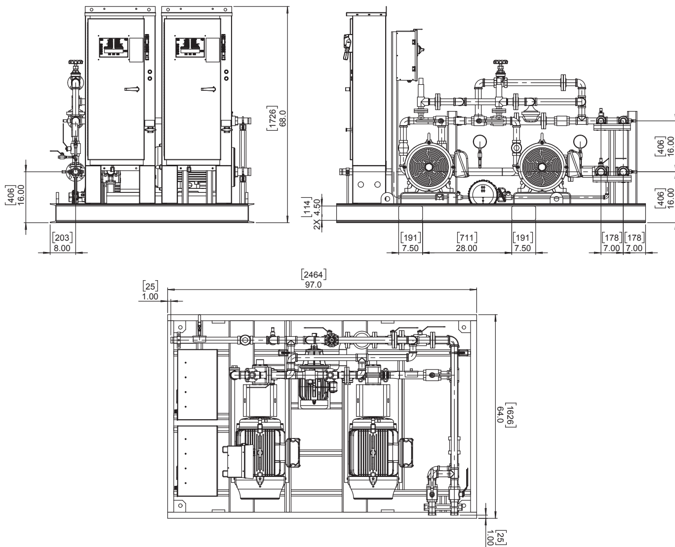
Figure 6.2.2: FoamPak 13D Dimensions
