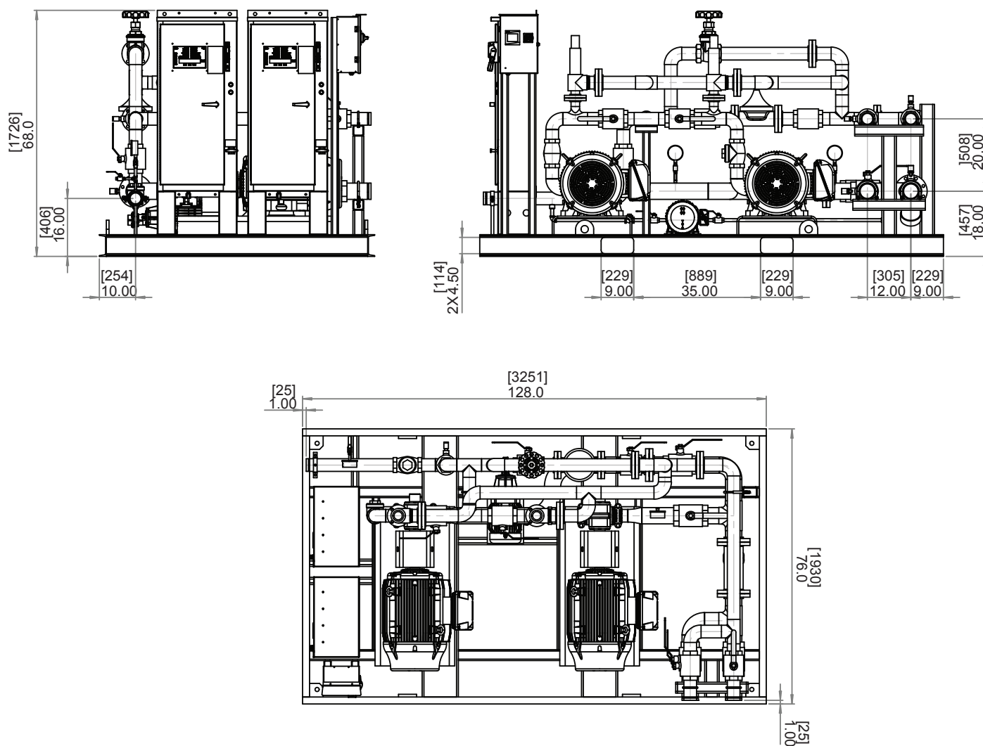
Figure 6.2.4: FoamPak 50D Dimensions
