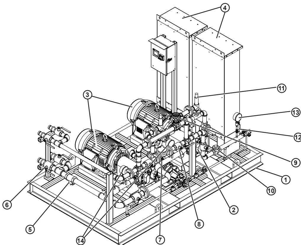
Figure 13.1.3: FoamPak 13D Components
