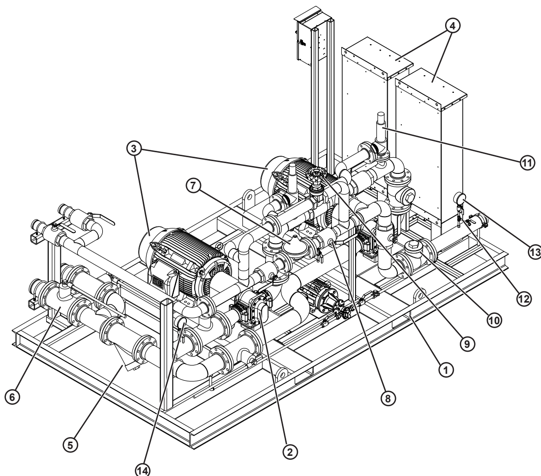
Figure 13.1.9: FoamPak 59D Components
