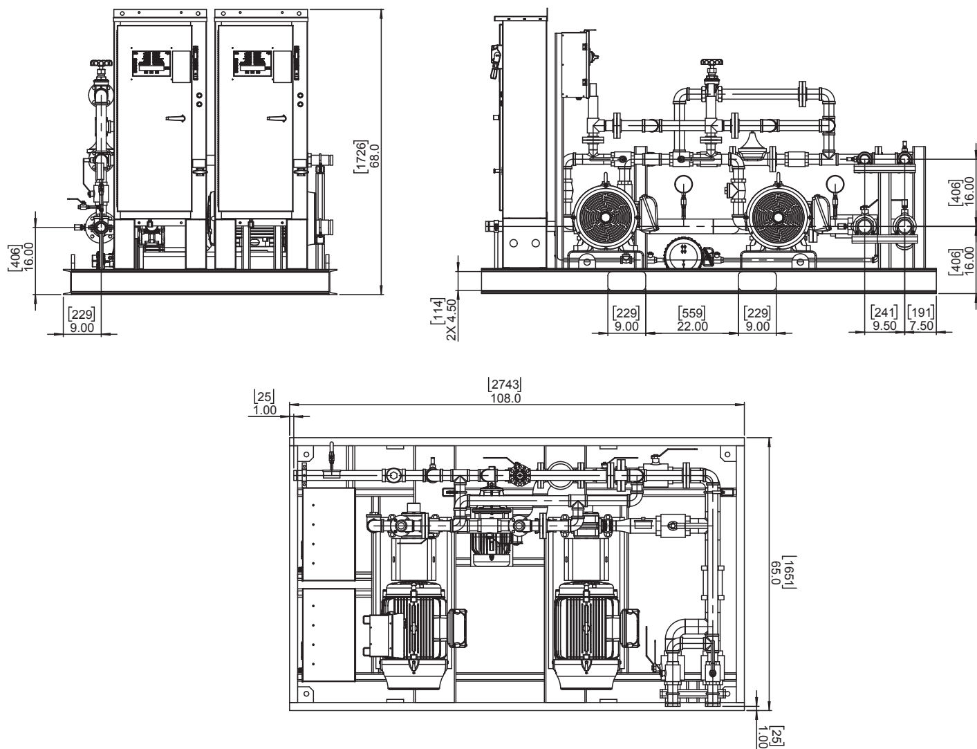
Figure 6.2.3: FoamPak 26D Dimensions
