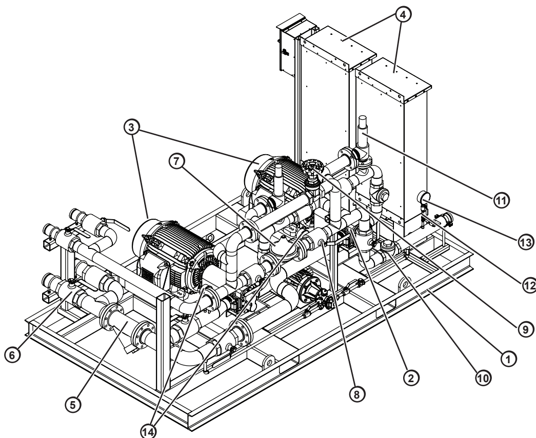
Figure 13.1.7: FoamPak 50D Components
