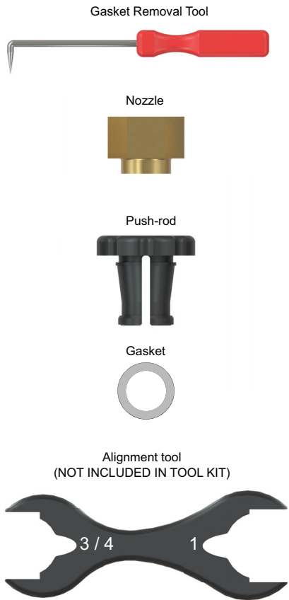
Figure – 1 Repair Kit Components
