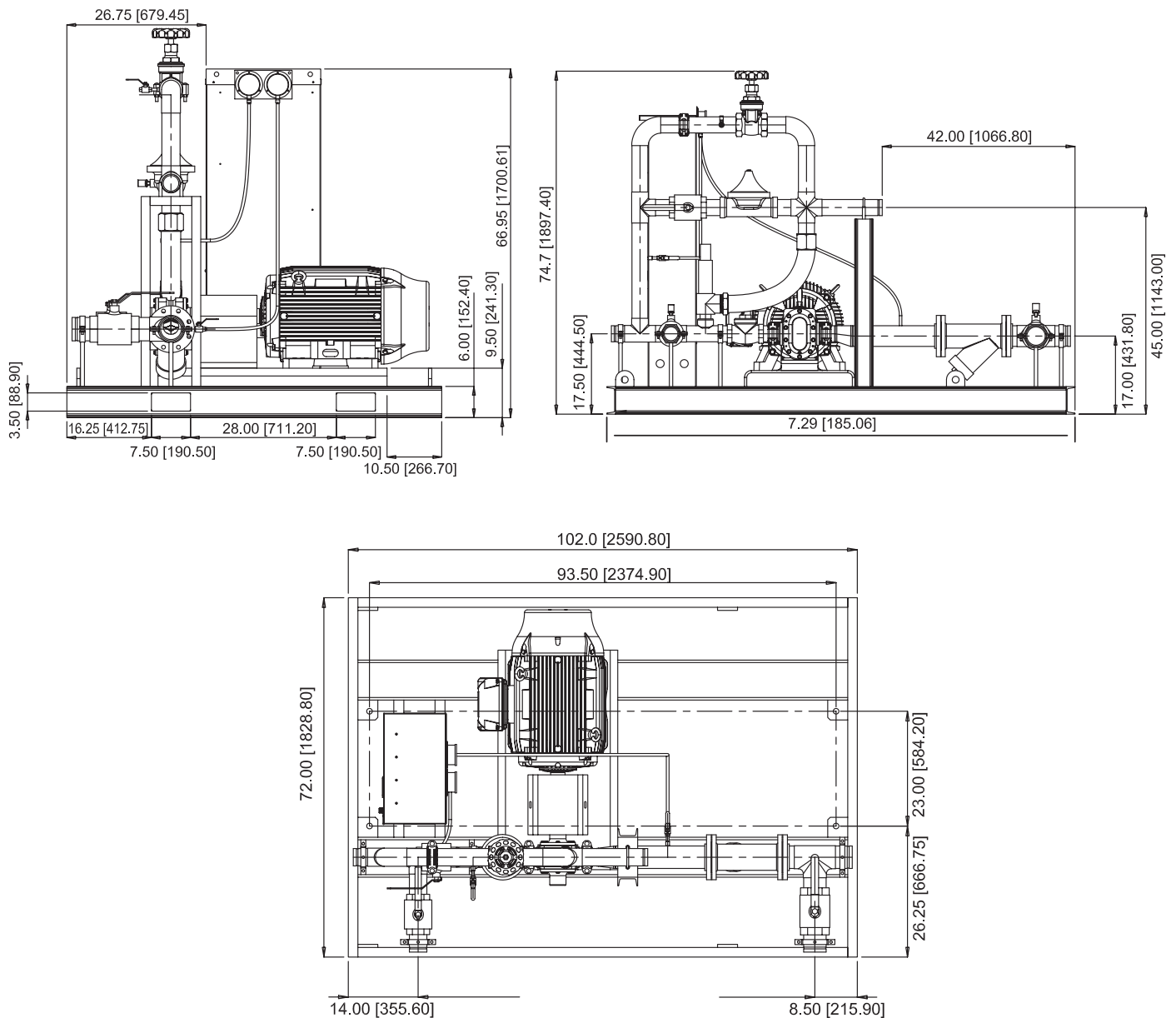
Figure 6.2.4: FoamPak 50S Dimensions
