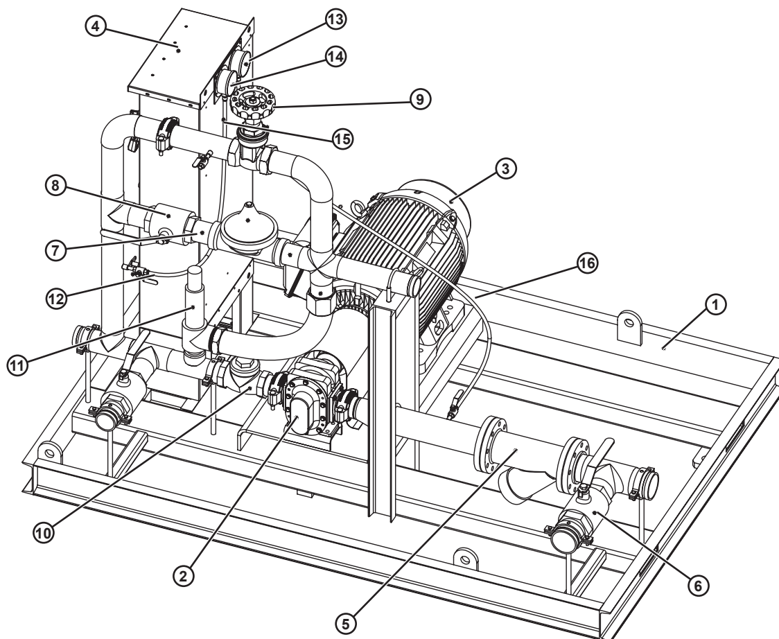
Figure 13.1.7: FoamPak 50S Components
