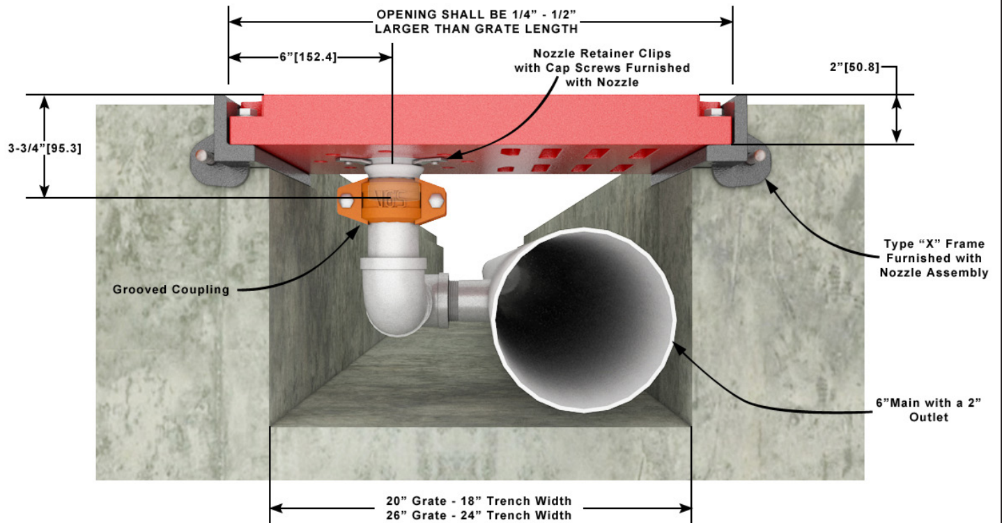
Figure 4 - Cross Section
