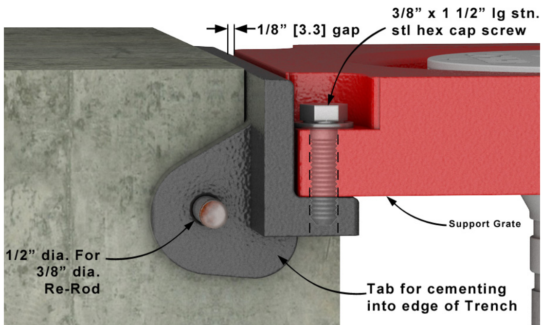
Figure 5 - X-Frame Detail
